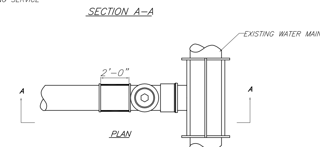
WATER SERVICE CONNECTION DETAIL N.T.S.
